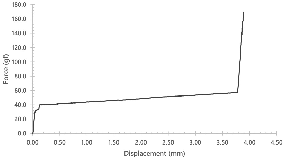
Keygeek Peach Cheesecake (48g) (Upstroke)
